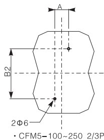
• CFM5-100~250 2/3P
