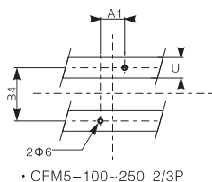
• CFM5-100~250 2/3P
