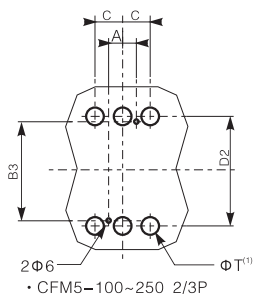
• CFM5-100~250 2/3P
