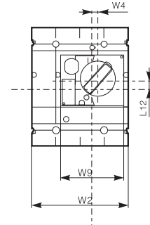
CFM5-100~630 4P Vigi CFM5-100~630 4P
