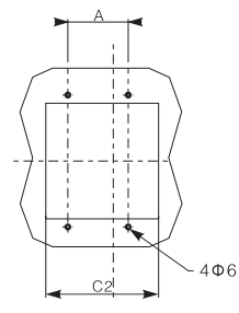
• CFM5-100~630 4P
