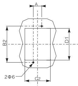
• CFM5-100~250 2/3P
