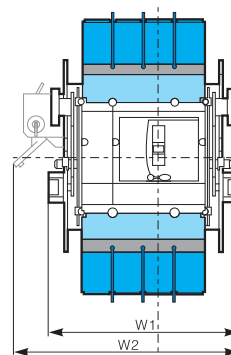
• CFM5-100~630 4P
