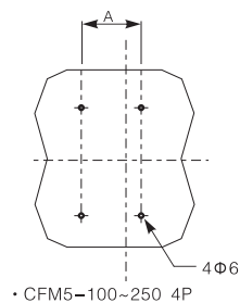
• CFM5-100~250 4P
