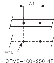
• CFM5-100~250 4P
