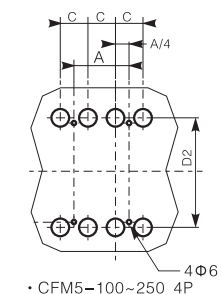
• CFM5-100~250 4P
