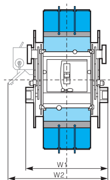
• CFM5-100~630 2/3P
